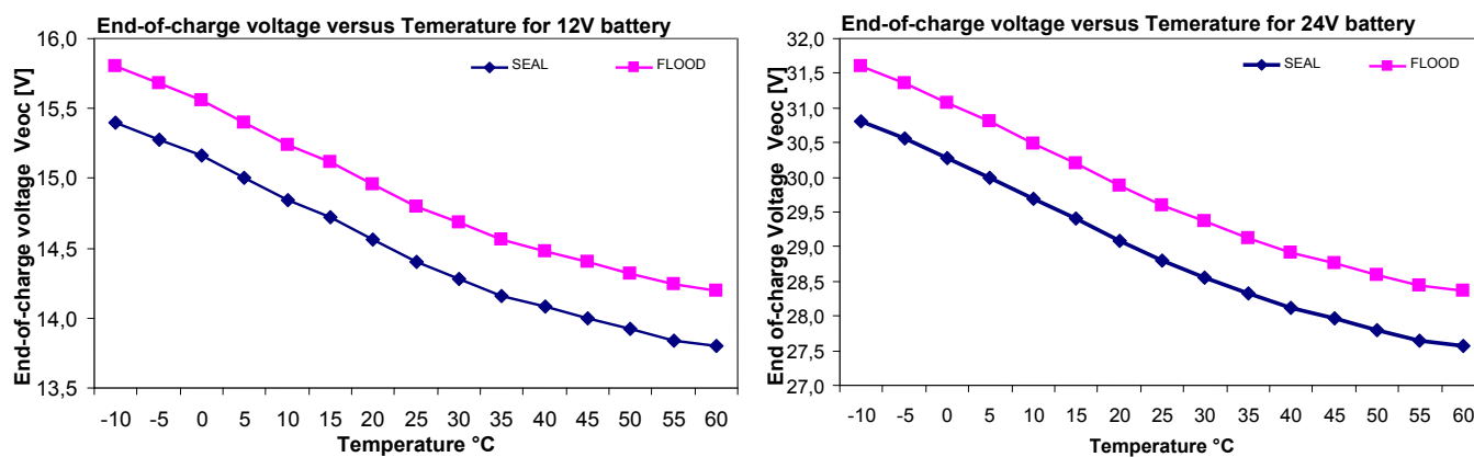
Pic. 6 Curve of the charging voltage compensation V_{ch} in function of battery temperature
