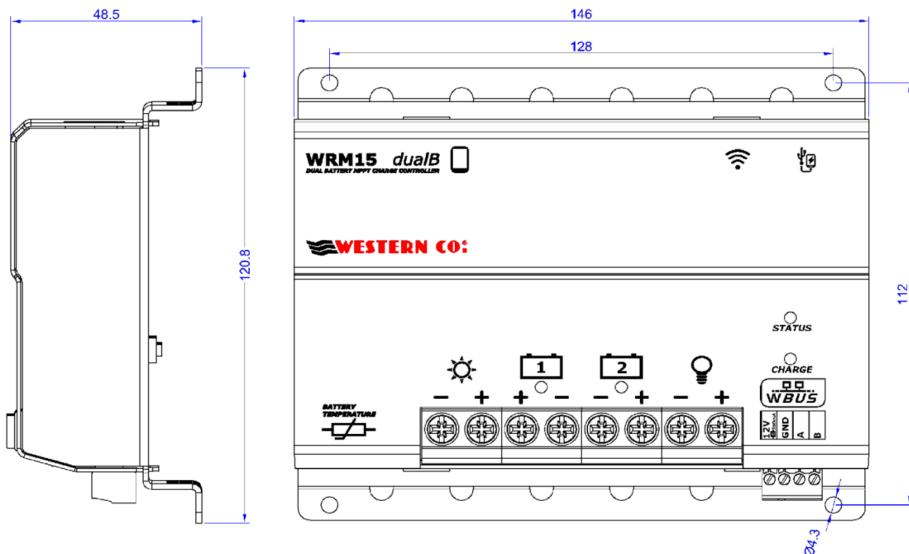
Pic. 5 Dimesions (mm)
